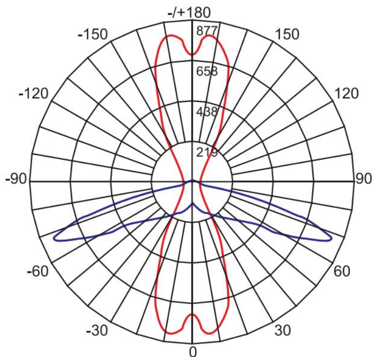
High Power LED Street Light LX-SL96
